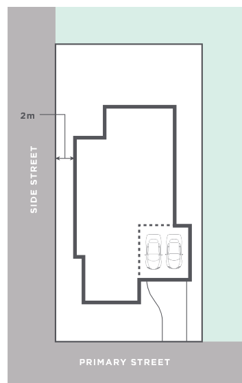
Side Setback
